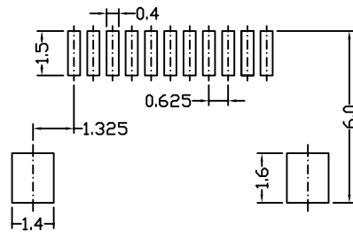
Recommand PCB Layout
