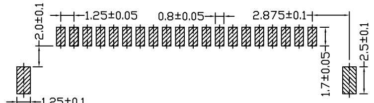
Recommand PCB Layout
