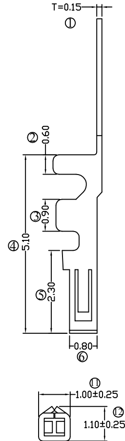
Section: C-C
